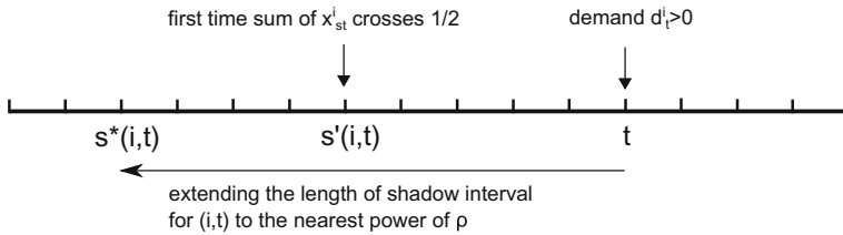
Fig. 1 Illustration of an extended shadow interval for demand point (i, t)
