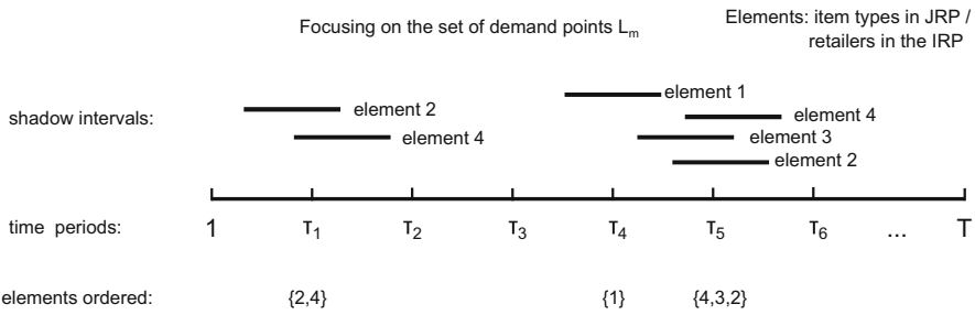
Fig. 2 Placing actual orders for the demand points within \mathcal{L}_m
