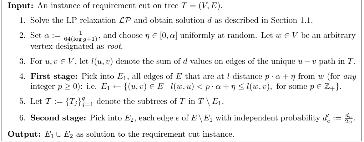
Figure 1: Algorithm for requirement cut on trees.
